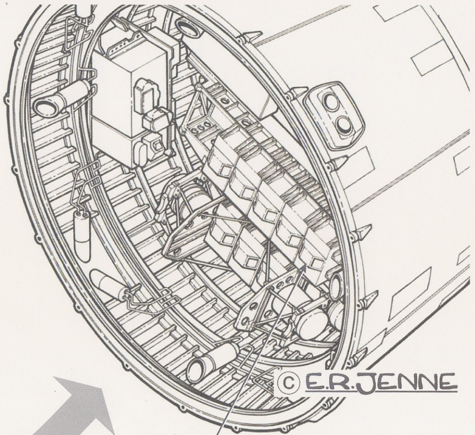
MODIFIED POWER SUPPLY ASSEMBLY (8 BATTERIES)
