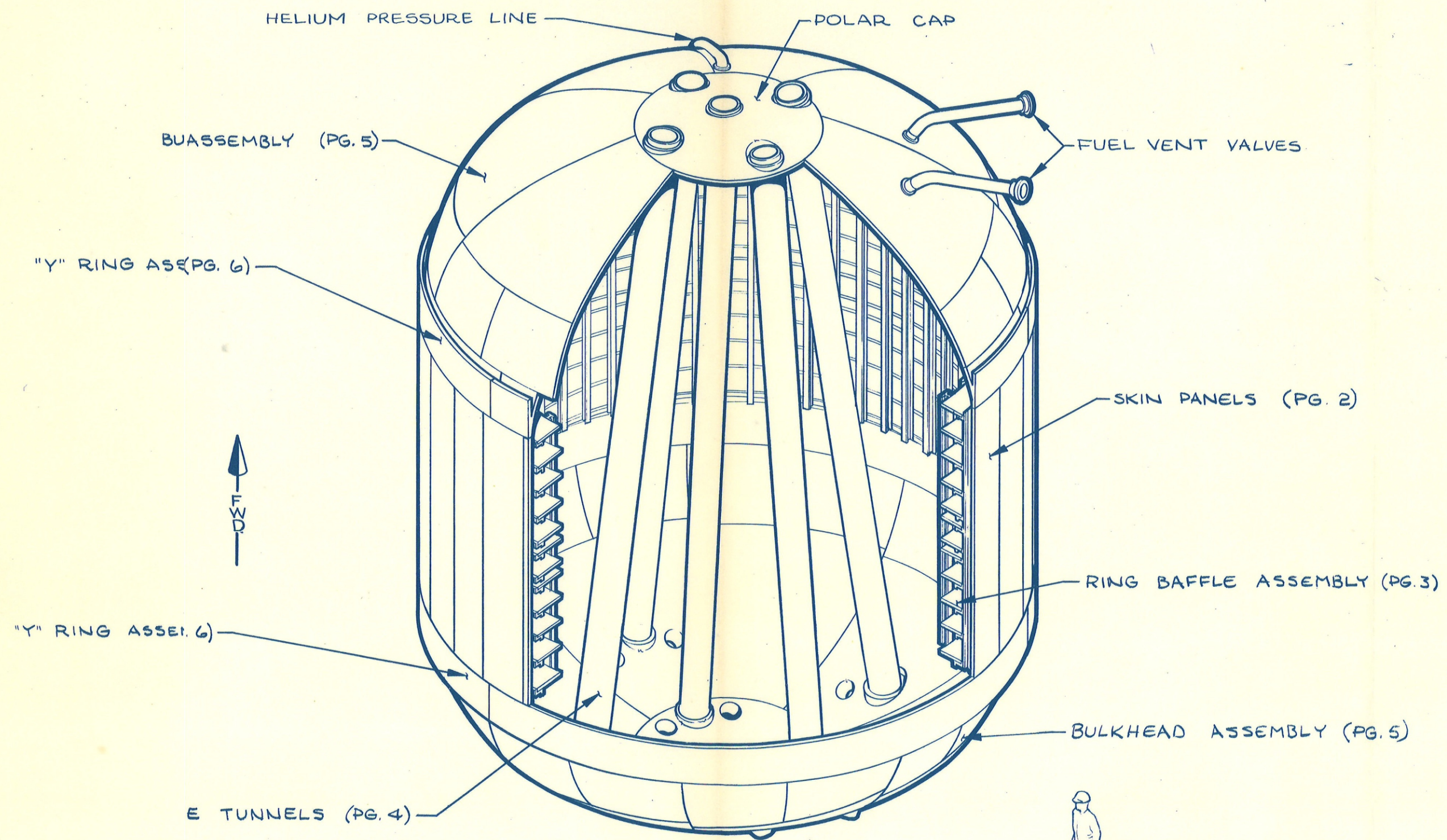
523-1103 FUEL TANK ASSEMBLY (PRELIMINARY SKETCH)
