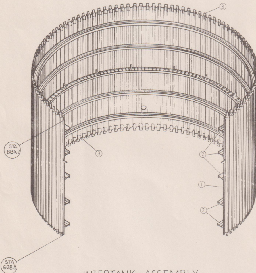
INTERTANK ASSEMBLY
