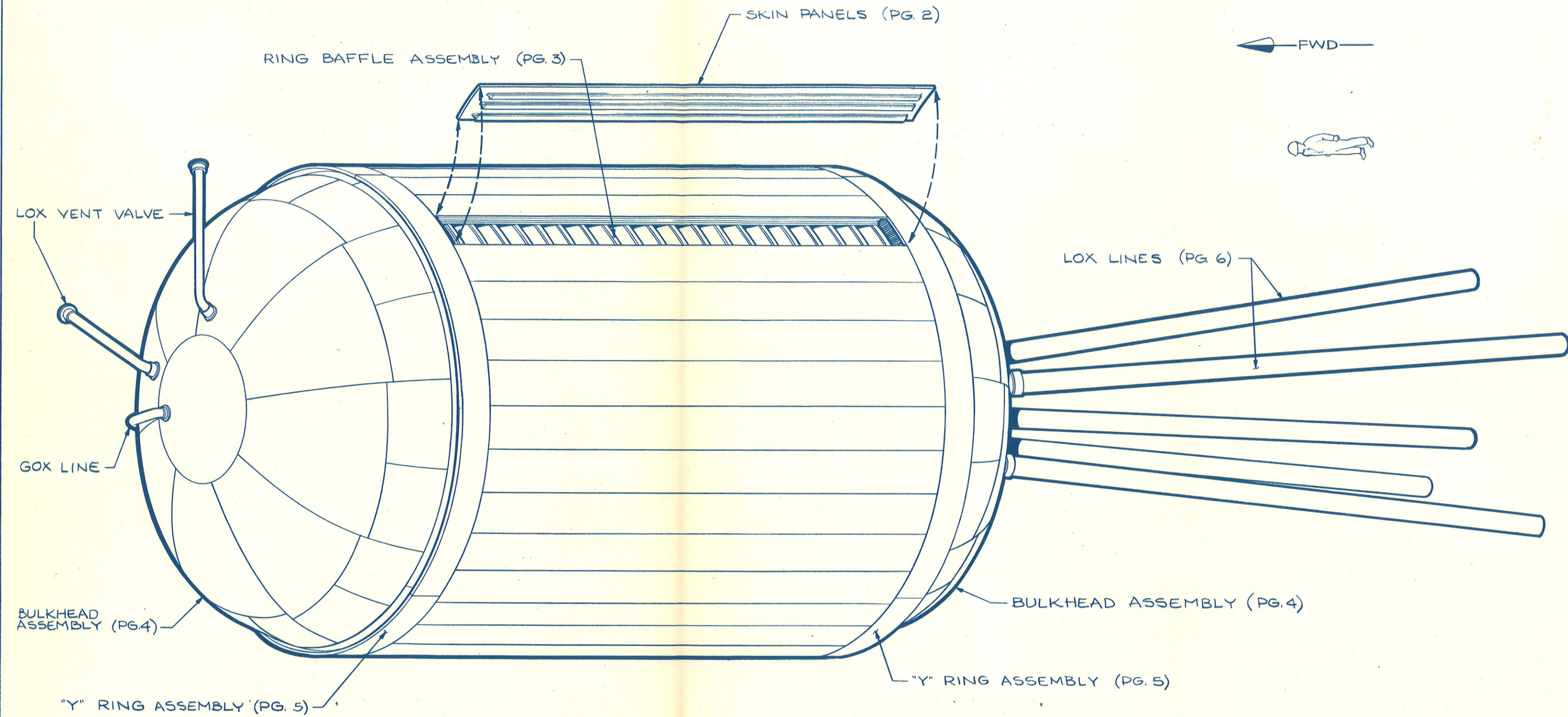
523-1105 LIQUID OXYGEN TANK (LOX TANK) (PRELIMINARY SKETCH)
