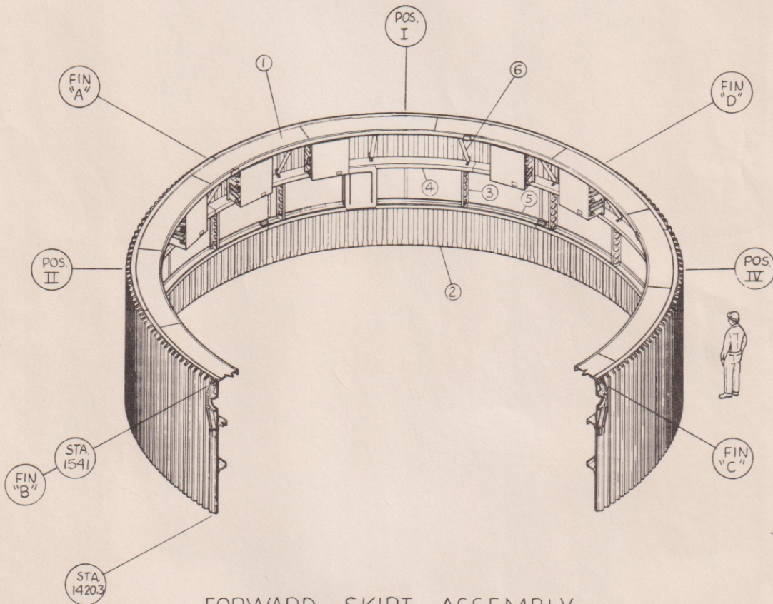
FORWARD SKIRT ASSEMBLY
